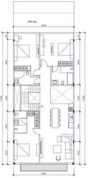
MẶT BẰNG TẦNG 3 CONSTRUCTION AREA: 127.3 m 2 BALCONY AREA: 5.5 m 2
