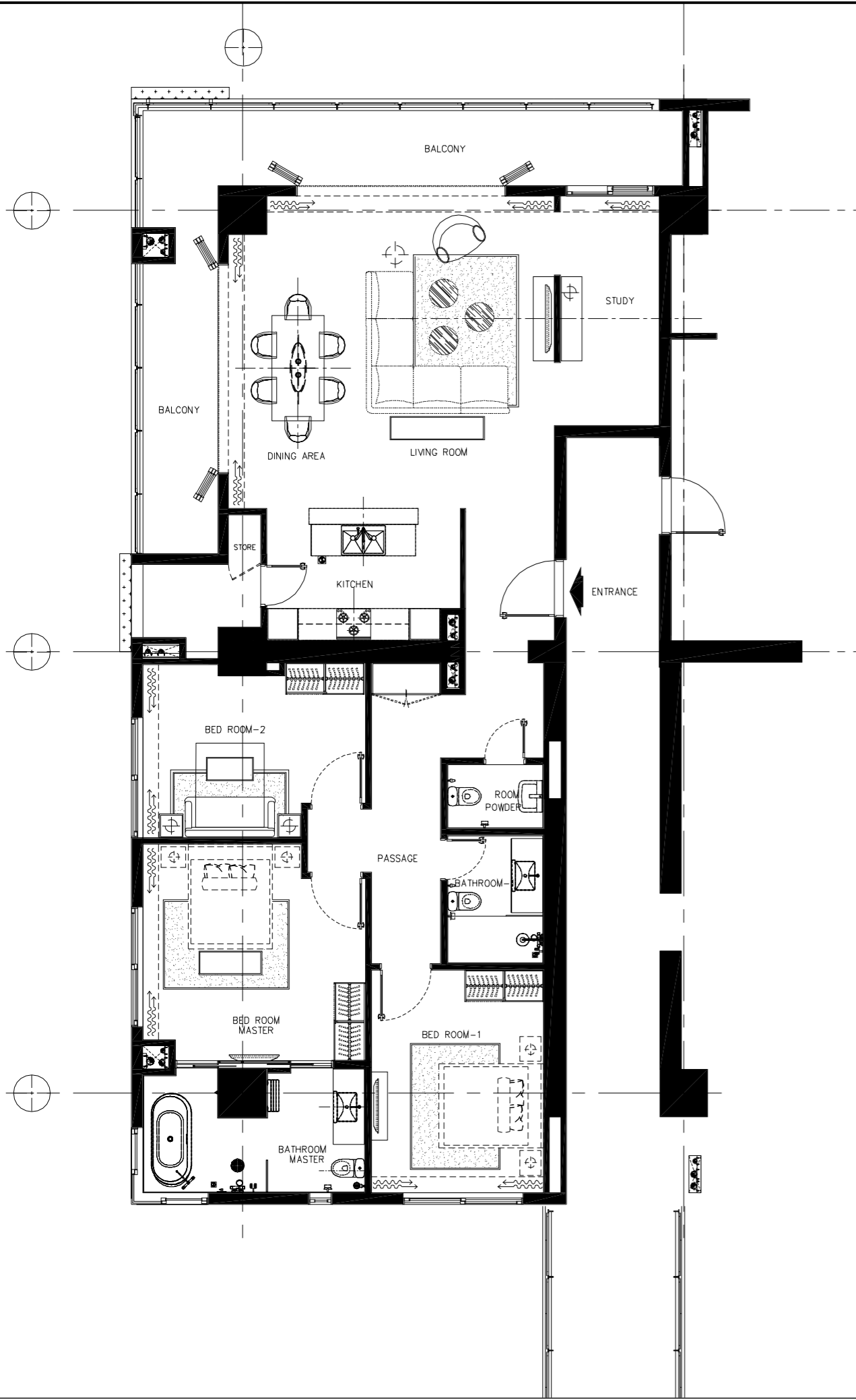
01 FF FIXTURE FURNITURE PLAN (FOR REFERENCE ONLY) Scale 1 : 50 (A1), 1 : 100 (A3)
