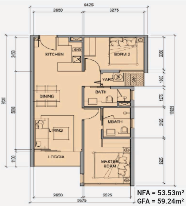
2BRM - REGULAR 2B
